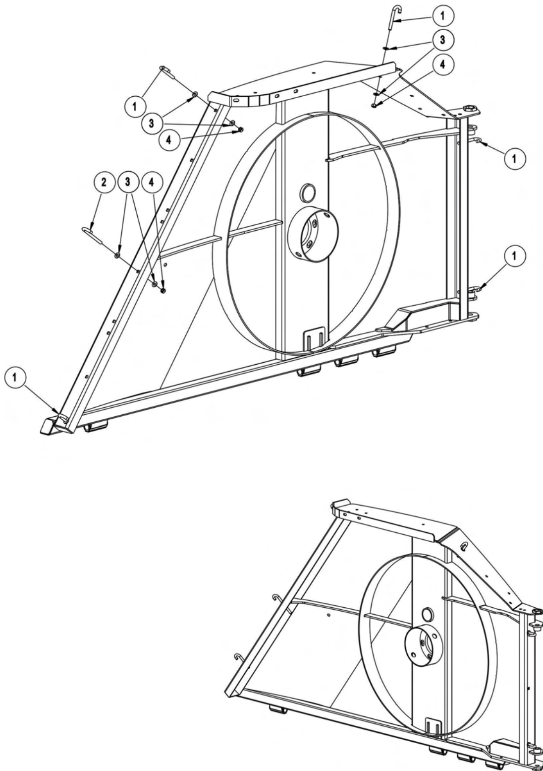
REAR VIEW
