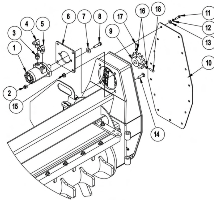
LOW FLOW DRIVE 8.0 CU. IN. MOTOR
