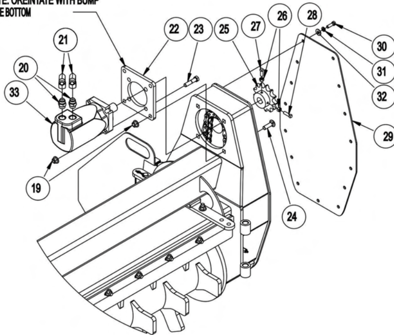
HIGH FLOW DRIVE 9.9 CU.IN., 15.0 CU.IN., 19.0 CU.IN. AND 24.0 CU. IN. MOTORS
